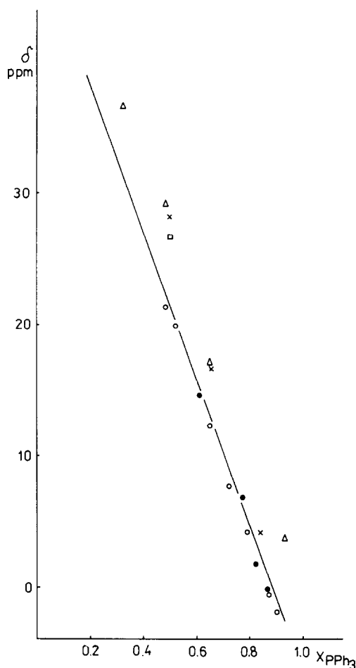
Fig. 1. Dependence of the ( \delta ) chemical shifts in the ^{31}P NMR spectra in C_6D_6 on mol fractions of the added phosphine X_{PPh_3} for complexes: [Rh(\beta\text{-diketone})(CO)(PPh_3)] where \beta -diketone: \circ ACA, \bullet BAC, \times NTA, \Delta BTA, \square TTA. The full line obeys the equation: 49.3(1 - X_{PPh_3}) - 6.1 X_{PPh_3} = \delta .
