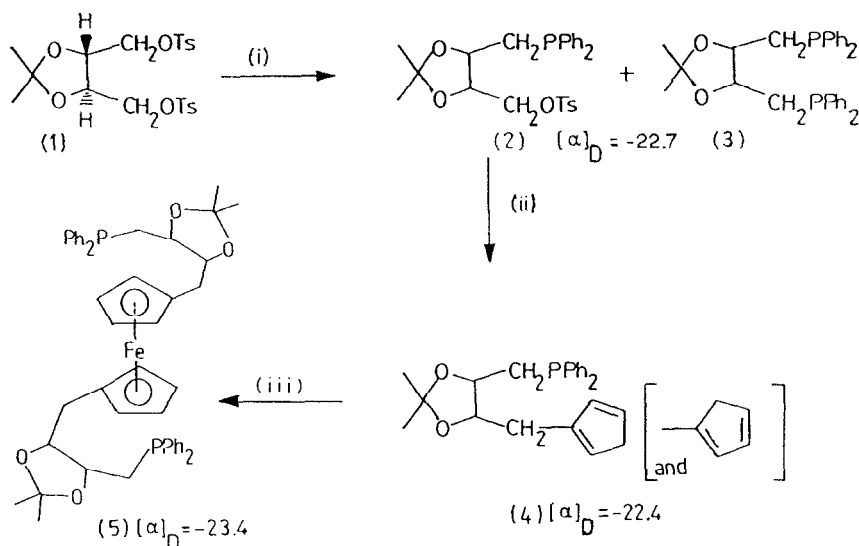
Scheme 1. For clarity hydrogens at the chiral centers are omitted after the first indication. (i) NaPPh 2 in THF at reflux for 6 h (27%). (ii) NaCp in THF at reflux for 4 h (58%). (iii) n-BuLi (1/1) in diethyl ether, at r.t. for 30 min, then FeCl 2 in THF at r.t. for 1 h (70%).
