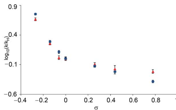
Fig. 1 Hammett plot for the second-order rate constants for the reaction outlined in Scheme 1 carried out at 289.6 K in either acetonitrile ( \blacktriangle ) or the ionic liquid [Bmim][N(CF 3 SO 2 ) 2 ] ( \bullet ).
