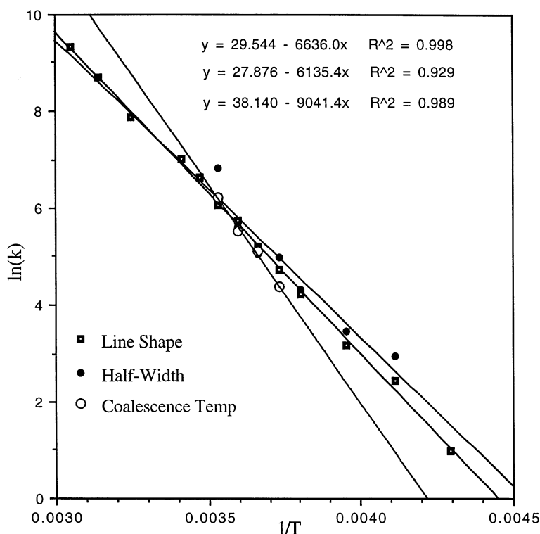
Fig. 7. Arrhenius plots for the rotational process illustrating the differences between the coalescence temperature measurements, the v_{1/2} approximation, and the complete line shape analysis.
