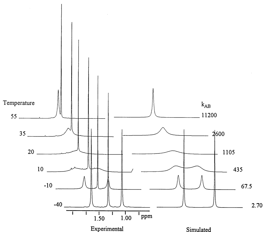
Fig. 5. A stacked plot showing the change in line shape of the 500 MHz 1 H-NMR spectrum as a function of temperature (left) and the simulated spectrum using a two-site model (right).
