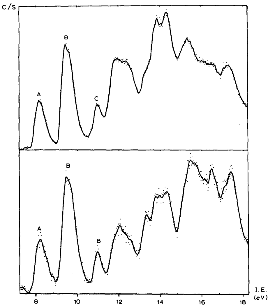
Fig. 2. HeI and HeII photoelectron spectra of (\text{C}_6\text{H}_5)(\text{C}_6\text{F}_5)\text{NH} .
