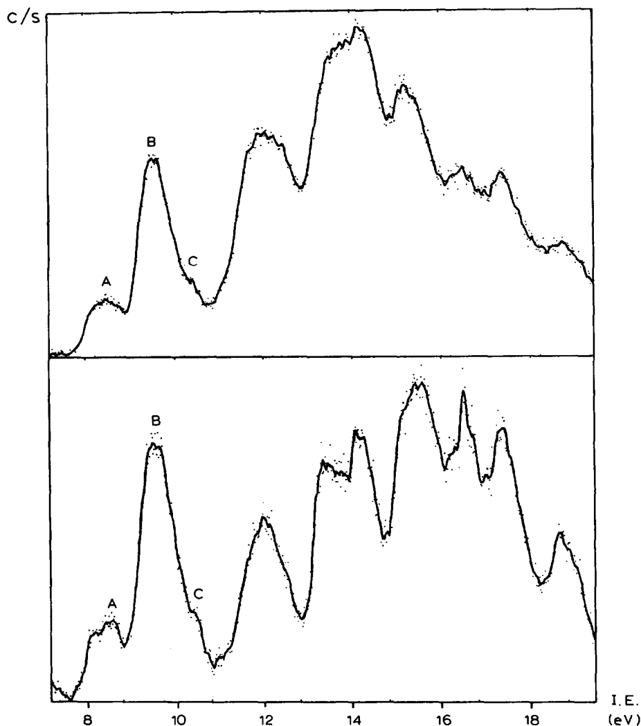
Fig. 4. Hel and HeI photoelectron spectra of [(C_6H_5)(C_6F_5)N]_2Si(CH_3)_2 .
