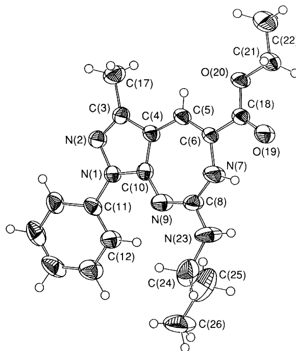
Fig. 2 Molecular structure of 6b . Selected geometrical parameters ( \text{\AA}^\circ ): C(4)–C(5) 1.451(6), C(5)–C(6) 1.331(7), C(6)–N(7) 1.402(7), N(7)–C(8) 1.337(7), C(8)–N(9) 1.294(6), N(9)–C(10) 1.348(6), C(10)–C(4) 1.385(6), C(4)–C(5)–C(6)–N(7) -1.3(9) , C(5)–C(6)–N(7)–C(8) -1.8(10) , C(6)–N(7)–C(8)–N(9) 0.4(11) , N(7)–C(8)–N(9)–C(10) 5.5(9) , C(8)–N(9)–C(10)–C(4) -8.9(9) , N(9)–C(10)–C(4)–C(5) 4.9(9) , C(10)–C(4)–C(5)–C(6) 1.2(8) , N(2)–N(1)–C(11)–C(16) -21.8(6) , C(5)–C(6)–C(18)–O(20) -6.6(7) , N(9)–C(8)–N(23)–C(24) -3.0(9) and N(23)–H(23)···O(19) (-x, 1 - y, -z) 0.92(7) , 2.01(7) , 2.929(6) , 176(7) .
