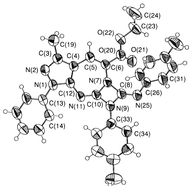
Fig. 1 Molecular structure of 3b . Selected geometrical parameters ( \text{\AA}^\circ ): C(4)–C(5) 1.455(3), C(5)–C(6) 1.335(4), C(6)–N(7) 1.421(4), N(7)–C(10) 1.417(3), C(10)–N(11) 1.265(3), N(11)–C(12) 1.391(4), C(12)–C(4) 1.376(4), N(7)–C(8) 1.439(4), C(8)–N(9) 1.418(4), N(9)–C(10) 1.389(3), C(8)–N(25) 1.250(3), C(4)–C(5)–C(6)–N(7) -6.8(4) , C(5)–C(6)–N(7)–C(10) 41.8(4) , C(6)–N(7)–C(10)–N(11) -40.9(5) , N(7)–C(10)–N(11)–C(12) 1.4(5) , C(10)–N(11)–C(12)–C(4) 19.1(4) , N(11)–C(12)–C(4)–C(5) 0.5(5) , C(12)–C(4)–C(5)–C(6) -17.5(5) , N(2)–N(1)–C(13)–C(18) 35.4(4) , C(5)–C(6)–C(20)–O(22) 38.1(4) , C(6)–N(7)–C(8)–N(25) 49.1(6) , N(7)–C(8)–N(25)–C(26) -0.8(6) , C(8)–N(25)–C(26)–C(27) 42.8(5) , N(11)–C(10)–N(9)–C(33) -17.6(5) and C(10)–N(9)–C(33)–C(38) -4.1(5) .
