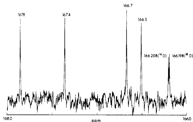
Figure 1. Natural abundance 100.6-MHz ^{13}\text{C} NMR spectrum of labeled [ 1-^{18}\text{O} ]-α-D-glucose pentaacetate in CDCl 3 . Chemical shift values are given in parts per million relative to Me 4 Si.
