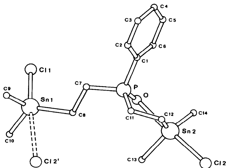
Fig. 2. Molecular structure of 1 with the atom-numbering scheme.
