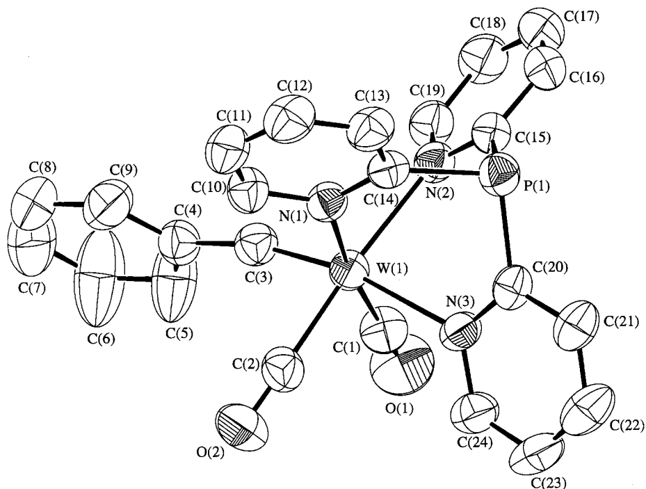
Fig. 2. Perspective view of [(\eta^3\text{-Ppy}_3)(\text{CO})_2\text{W}\equiv\text{CPh}]^+ (40% probability ellipsoids).
