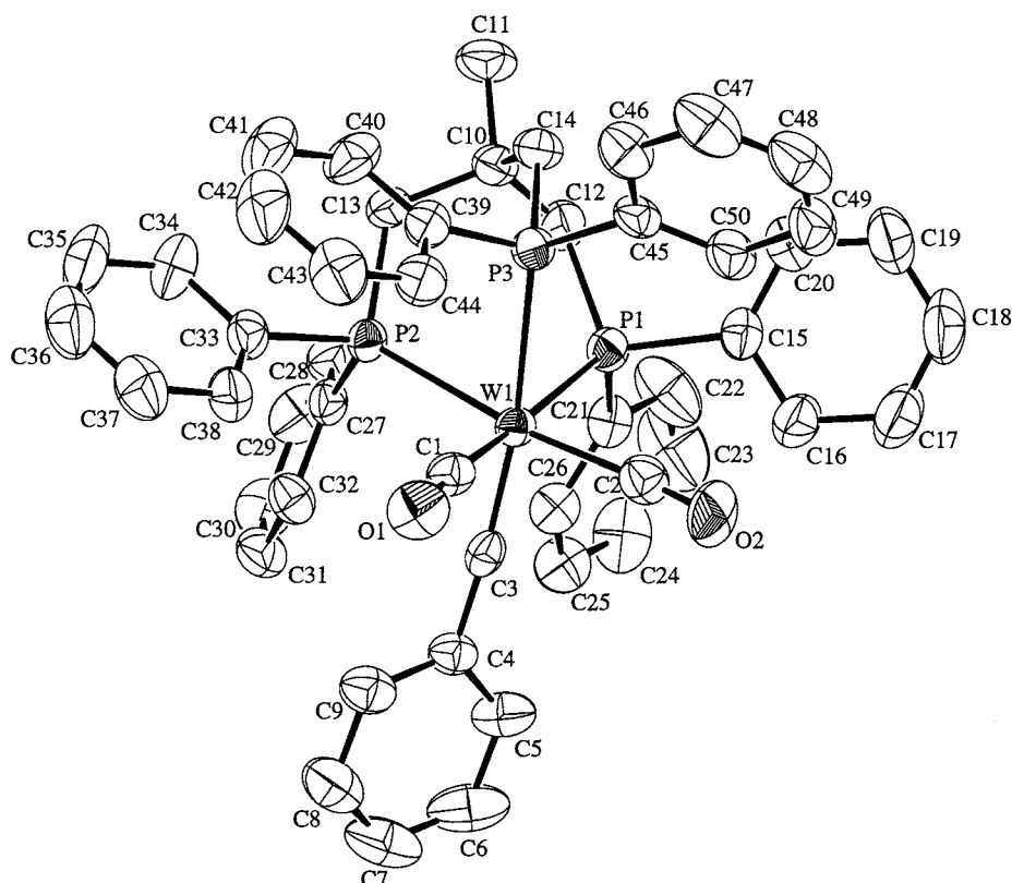
Fig. 4. Perspective view of [\{\text{CH}_3\text{C}(\text{CH}_2\text{PPh}_2)_3\}(\text{CO})_2\text{W}\equiv\text{CPh}]^+ (40% probability ellipsoids).
