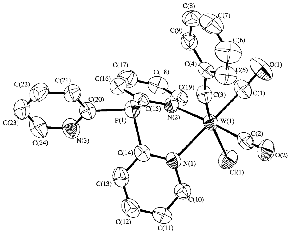
Fig. 1. Perspective view of [\text{Cl}(\eta^2\text{-Ppy}_3)(\text{CO})_2\text{W}\equiv\text{CPh}] (40% probability ellipsoids).
