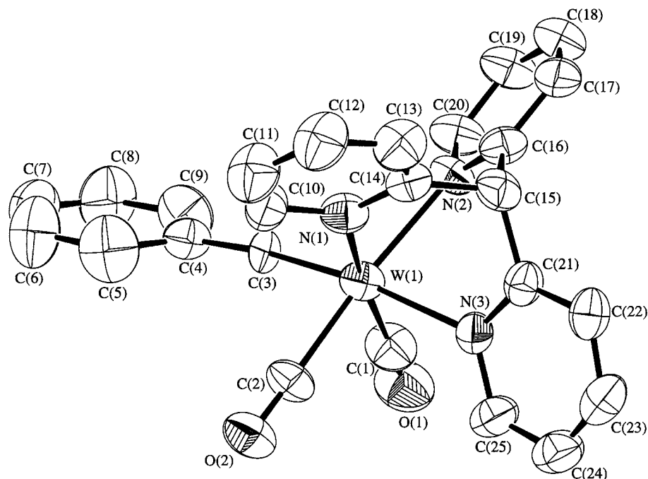
Fig. 3. Perspective view of [(\eta^3\text{-HCpy}_3)(\text{CO})_2\text{W}\equiv\text{CPh}]^+ (50% probability ellipsoids).
