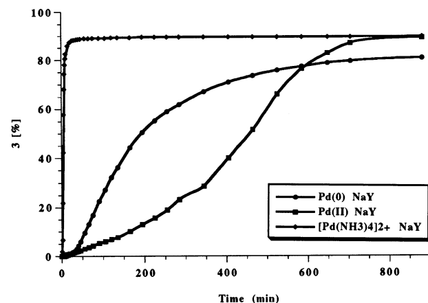
Fig. 4. Kinetic investigations: comparison of the activity of different Pd-species loaded into the zeolites. Percentage of the product 3 obtained with the [\text{Pd}(\text{NH}_3)_4]^{2+} -, Pd(II)- and Pd(0)-loaded NaY for the Heck reaction (Scheme 1).
