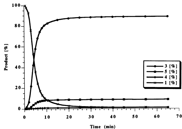
Fig. 3. Kinetic investigations: Conversion of bromofluorobenzene 1 and product percentage ( 3 , 4 and 5 ) obtained with the [\text{Pd}(\text{NH}_3)_4]^{2+} -loaded NaY for the Heck reaction (Scheme 1).
