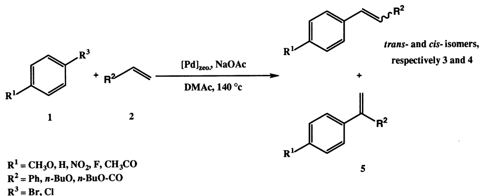
Scheme 2. Reaction conditions: 10 mmol aryl halide 1, 15 mmol olefin 2, 15 mmol NaOAc, 0.1 mol% [\text{Pd}]_{\text{zeo}} , 8 ml DMAc, 140°C, 20 h.
