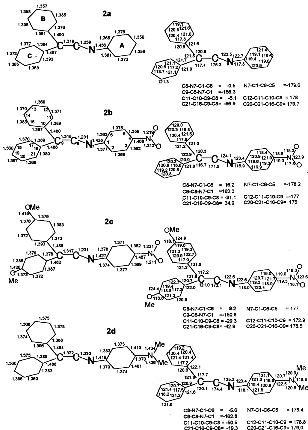
Figure 2. Crystallographic data of four ketenimine derivatives.
