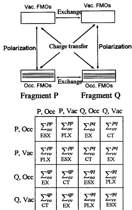
Figure 6. Morokuma's definitions of the FMO interactions between fragments P and Q (P, Q = A, B, C).
