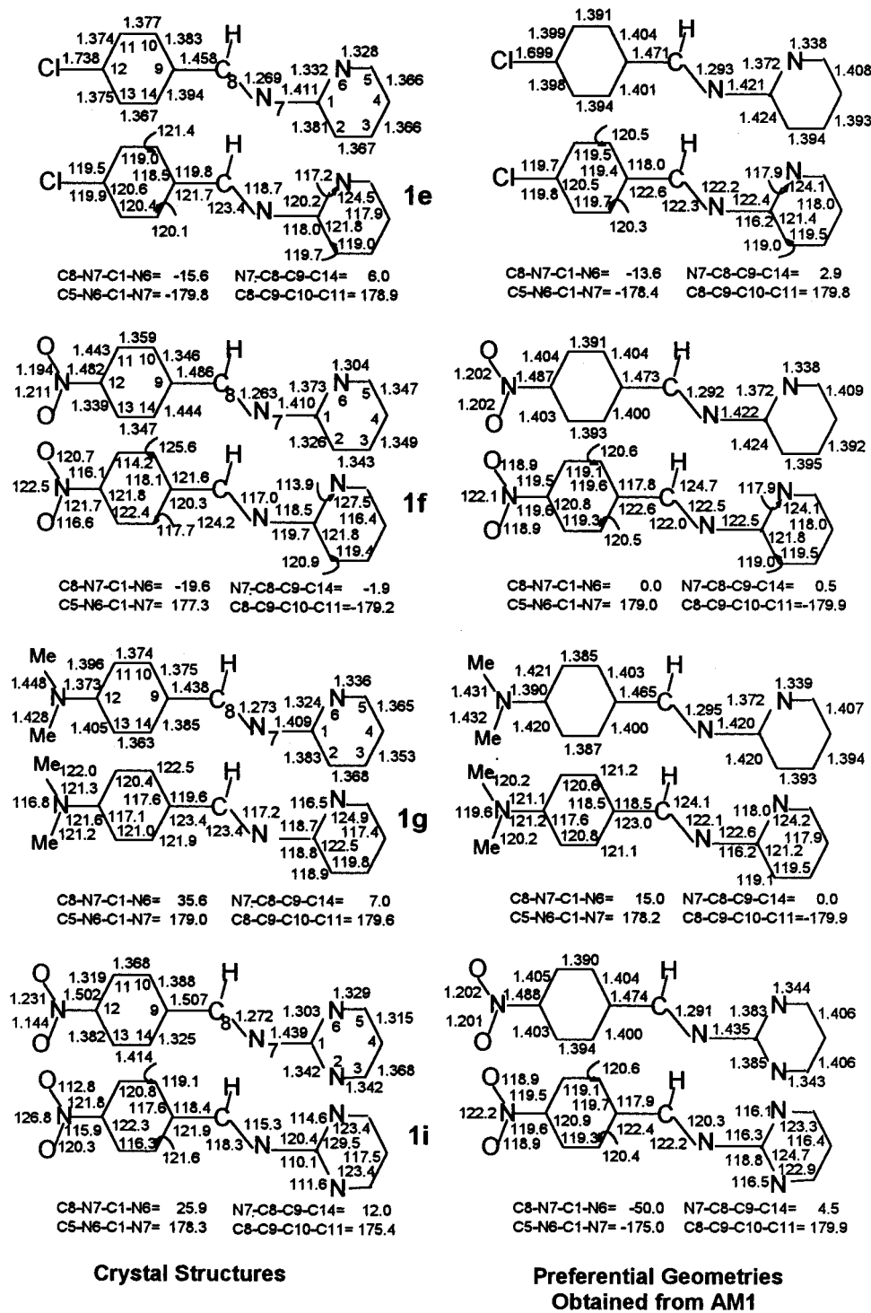
Figure 1. Experimental and theoretical geometric data of four stilbene-like molecules.
