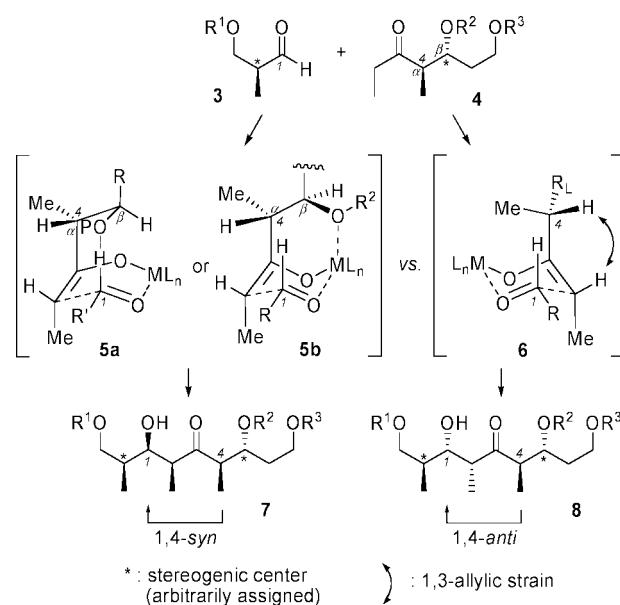
Scheme 1. Working Model for Diastereodivergent 1,4- syn versus 1,4- anti Aldol Coupling (Exemplarily Shown for Z-Enolates 5/6 )
