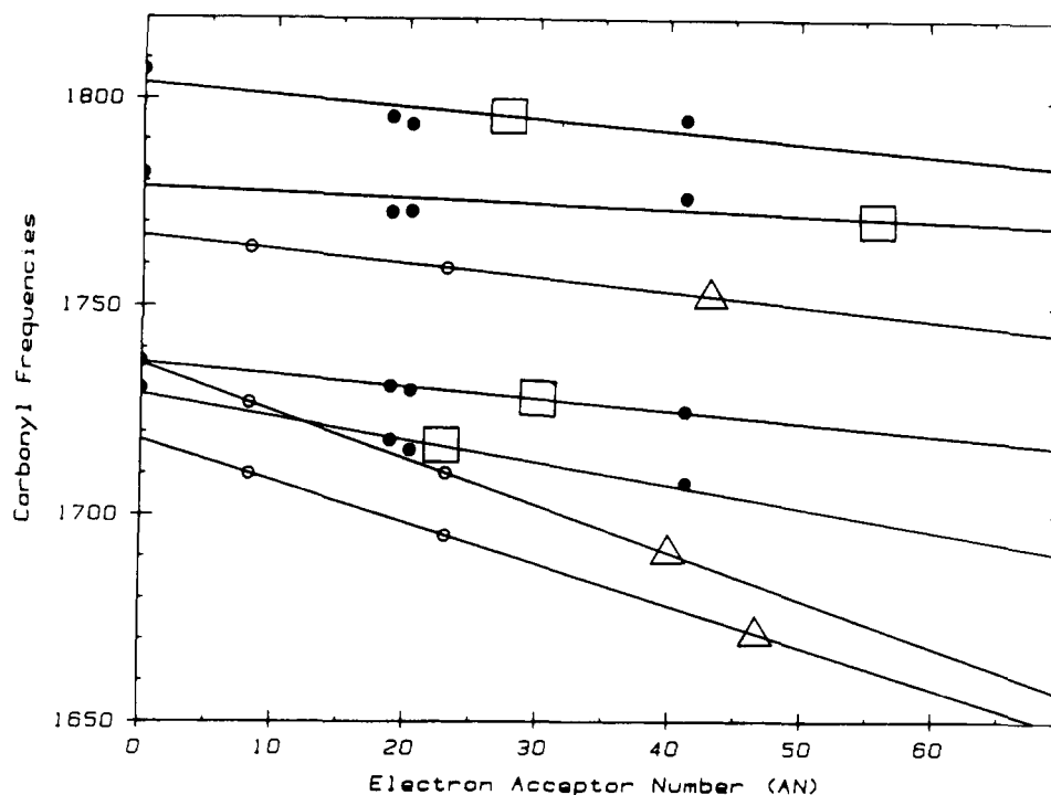
Figure 7. Correlation of the \nu > 1650 \text{ cm}^{-1} bands from the interaction of DA and PLA with CPA to the plots of \nu(\text{C}=\text{O}) for DAA, Zn(II)-complexed DAA, and DA. Large open squares denote bands from the back-reaction that are attributed to an anhydride intermediate. Open triangles denote bands that are attributed to a Zn(II)-complexed anhydride intermediate.
