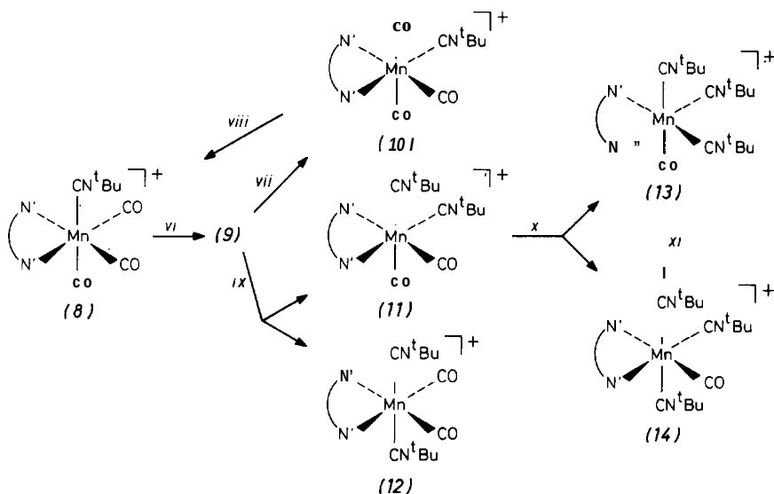
Scheme 2. N'-N' = {}^t\text{Bu-DAB} or \text{tmed} ; (vi) \text{ONMe}_3 ; (vii) \text{CO} ; (viii) refluxing hexane for 10a , or stirring at room temperature for 10b , (ix) \text{CN}^t\text{Bu} ; (x) \text{ONMe}_3 and \text{CN}^t\text{Bu} ; (xi) refluxing \text{CHCl}_3 , only for 13b
