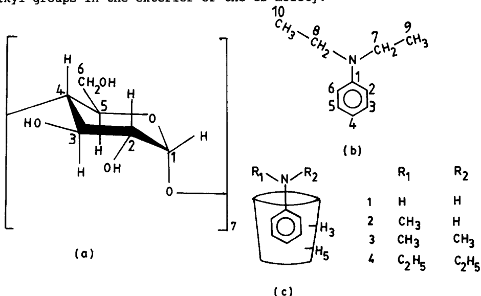
Figure 1. Structures of (a) \beta -CD, (b) DEA and (c) postulated conformations of \beta -CD-aniline complexes.
