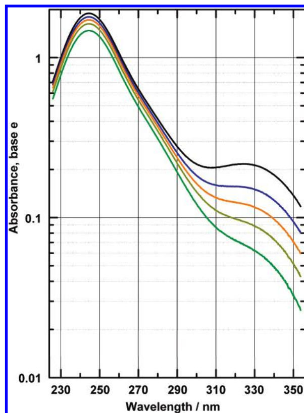
Figure 2. Absorbance vs wavelength for spectra using method 1 to generate chlorine peroxide. The strong peak near 245 nm is due to ClOOC1 and the shoulder at 330 nm is caused by \text{Cl}_2 . Each spectrum is for a 5 s integration time. These five spectra, with time increasing from top to bottom, were collected during a 2.4 min period.
