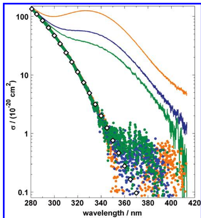
Figure 9. Cross sections at longer wavelengths for three spectra using method 1 to generate ClOOCl. Conditions as in Figure 2. The fitted ratios of Cl 2 /ClOOCl are 4.46, 1.86, and 1.13 for the top three spectra. Using the same color code, the lower points result from subtracting out the contributions from \sigma(\text{Cl}_2) . The open diamonds are \sigma(2\text{Gauss}) from eq 17.
