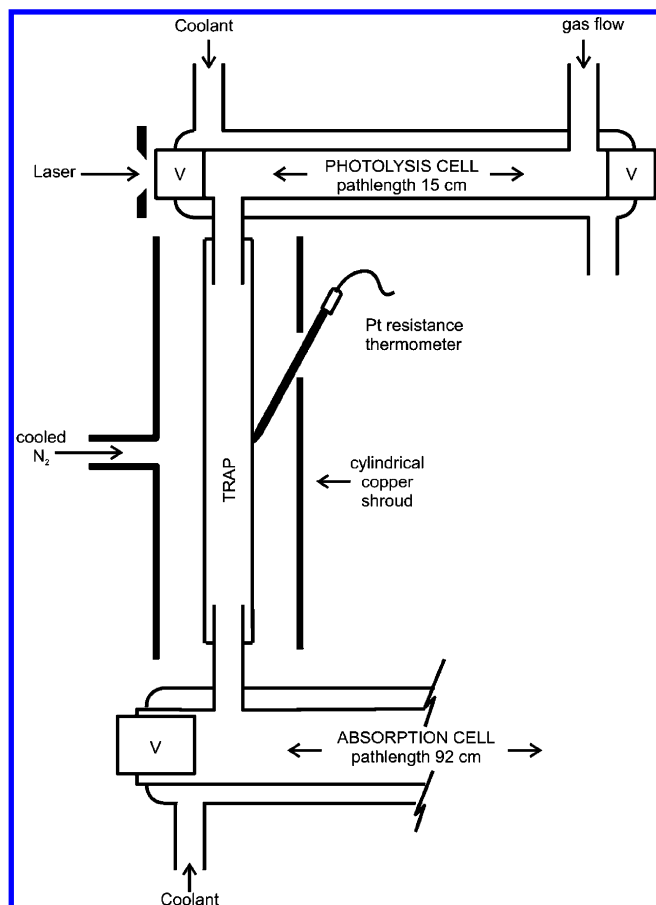
Figure 1. Diagram of the photolysis cell, trap and absorption cell. Quartz was used for all surfaces in contact with the gas stream. V indicates evacuated chambers to avoid water condensation on the windows. The UV analysis beam made two passes through the absorption cell, for a total path length of 184 cm.
