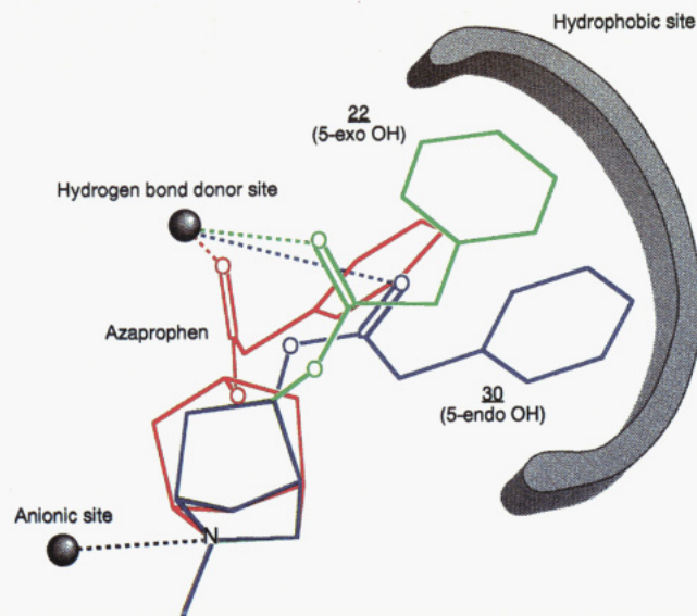
Figure 1. Schematic drawing of the alignment of azapropen, compound 22, and compound 30 to the proposed muscarinic pharmacophore. All protons, the methyl, and one phenyl group of the ester side chain are not shown for clarity.
