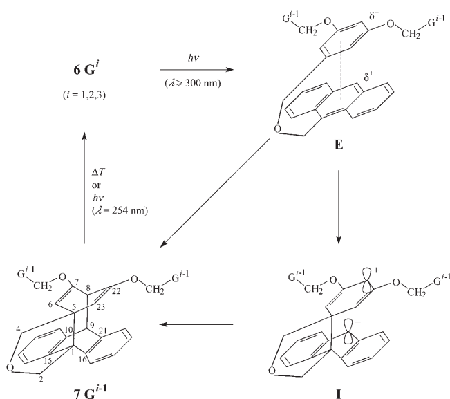
Scheme 5. Intramolecular [4\pi+4\pi] cycloaddition and cycloreversion 6\text{G}^i \rightleftharpoons 7\text{G}^{i-1} .
