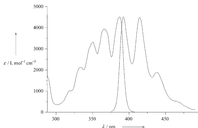
Figure 1. Long-wavelength absorption and normalized fluorescence band ( \lambda_{\text{exc}} = 260 \text{ nm} ) of 6G 2 in \text{CH}_2\text{Cl}_2 .
