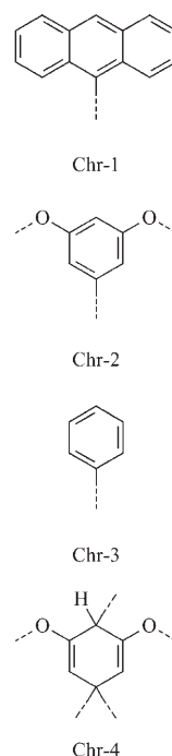
Scheme 7. Photophysical and photochemical process of the dendrimers 6G i ( i = 1–3) with chromophores Chr-1,2,3 and their cyclomers 7G i-1 with chromophores Chr-2,3,4: A: Absorption, \lambda_1 \geq 300 nm, \lambda_2 = 254 or 260 nm; F: Fluorescence; IC: Internal conversion; ET: Singlet energy transfer; PhR: Photoreaction.
