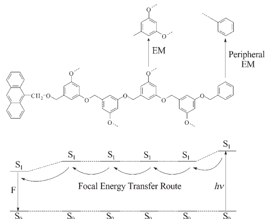
Scheme 6. Downhill focal energy-transfer (ET) route in the dendrimers 6G i and competing peripheral energy migration (EM).
