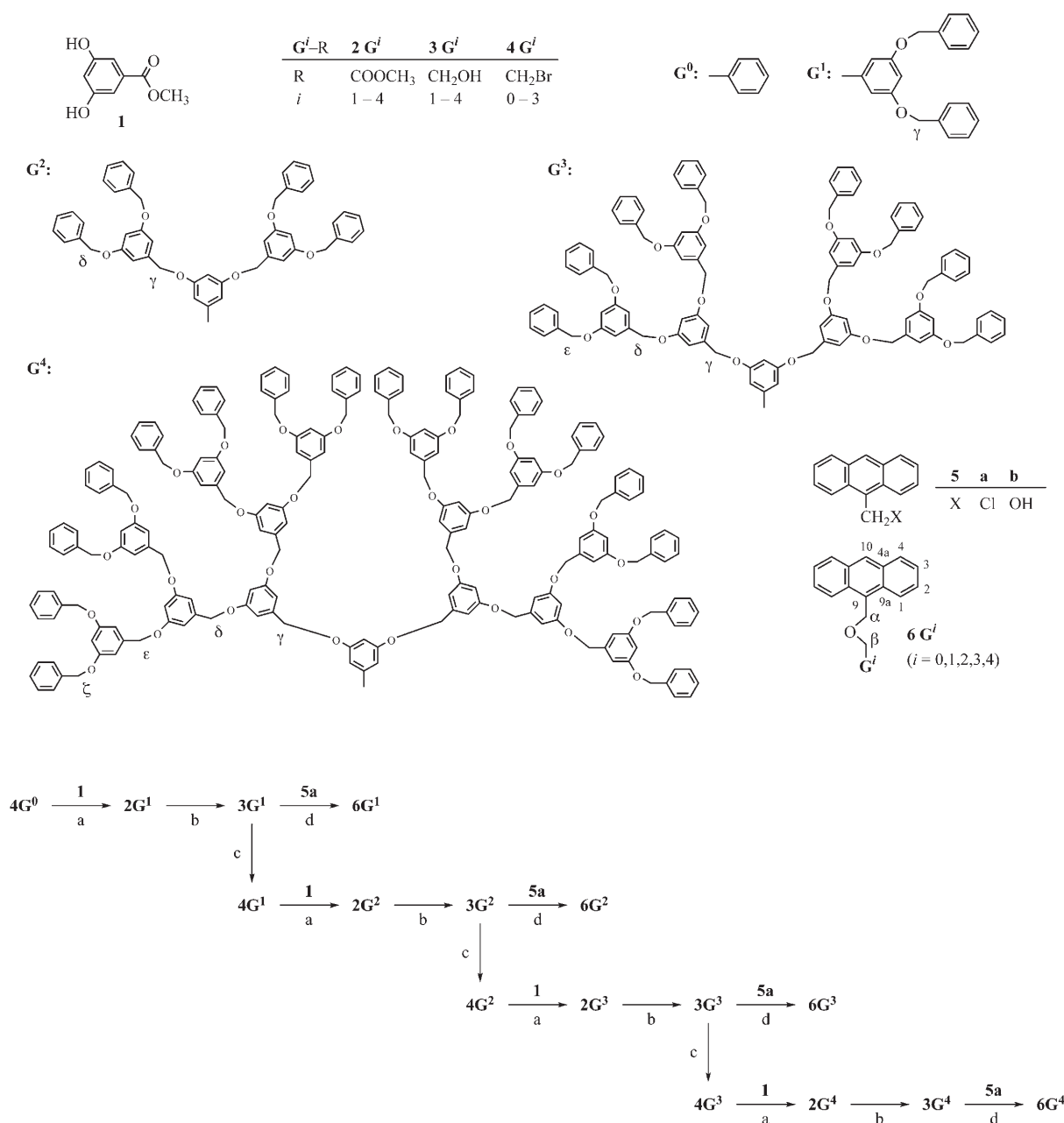
Scheme 2. Structures of the target dendrimers 6G^i ( i=1-4 ), their precursors 1 , 2G^i , 3G^i , 4G^i , 5a , and model compounds 6G^0 and 5b . Preparation mode of 6G^i . a) K_2CO_3 , Me_2CO ; b) LiAlH_4 , THF; c) PBr_3 , C_6H_5CH_3 ; d) (nBu)_4N^+Br^- , C_6H_5Cl/KOH , H_2O .
