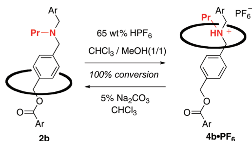
Scheme 1. Shuttling Behavior of [2]Rotaxane 2b / 4b • \text{PF}_6 based on the Treatment with Acid/Base
