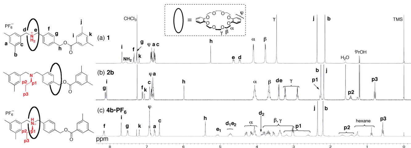
Figure 1. ^1\text{H} NMR spectra of (a) sec -ammonium salt-type rotaxane 1 , (b) tert -amine-type rotaxane 2b , and (c) tert -ammonium salt-type rotaxane 4b • \text{PF}_6 (400 MHz, \text{CDCl}_3 , 298 K).
