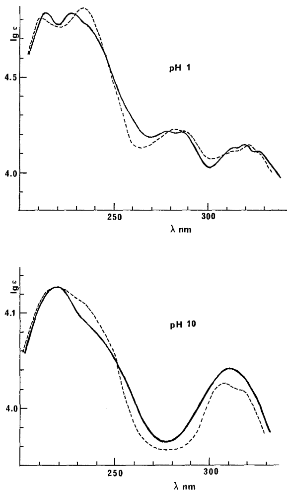
Abb. 1. UV-Absorptionsspektren von 3-Benzyl-4-hydroxy-1-(2-pyridyl)-chinolin-2(1 H )-on 1 : —; 3-Benzyl-1-(2-chinolinyl)-4-hydroxy-chinolin-2(1 H )-on ( 6 ): — (1 × 10 -5 M)
