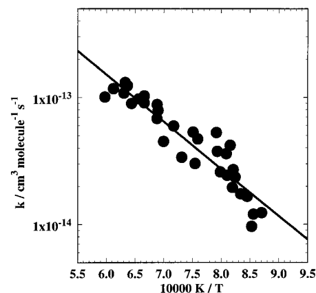
Figure 3. Arrhenius plot of the data from Table 1. The line is given by eq 5, and the solid circles are the individual data points.
