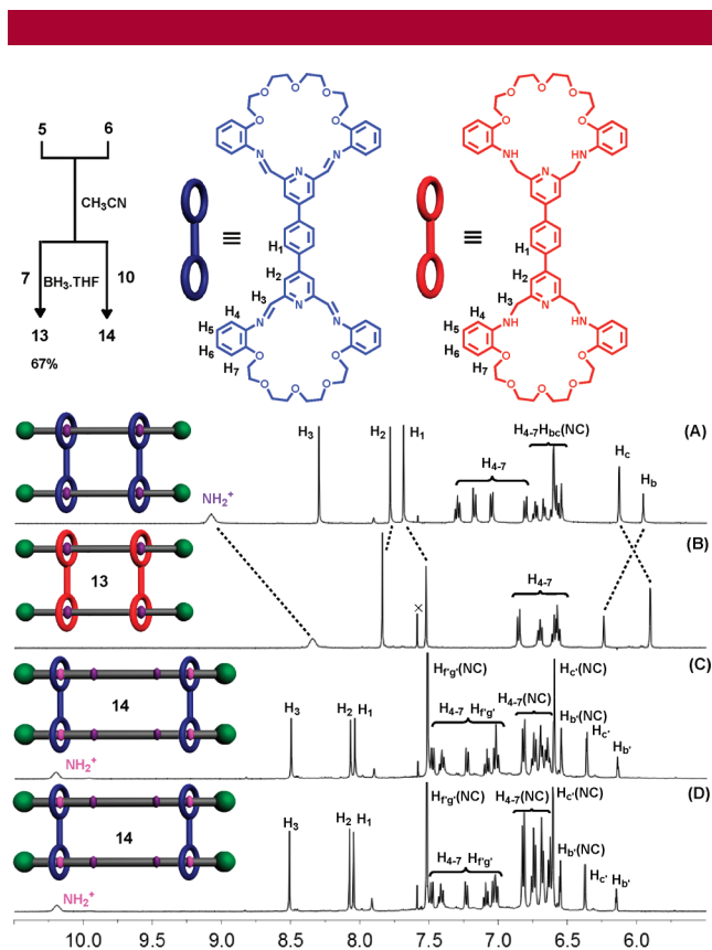
Figure 4. Partial ^1\text{H} NMR spectra (500 MHz in \text{CD}_3\text{CN} at rt) of the rectangular dynamic [4]rotaxane based on 7 (A); the kinetically stable [4]rotaxane 13 (B); the dynamic [4]rotaxane 14 when the ratio of 5/6/10 = 2:1:1 (C); and the dynamic [4]rotaxane 14 when the ratio of 5/6/10 = 4:2:1 (D). (NC indicates noncomplexed components.)
