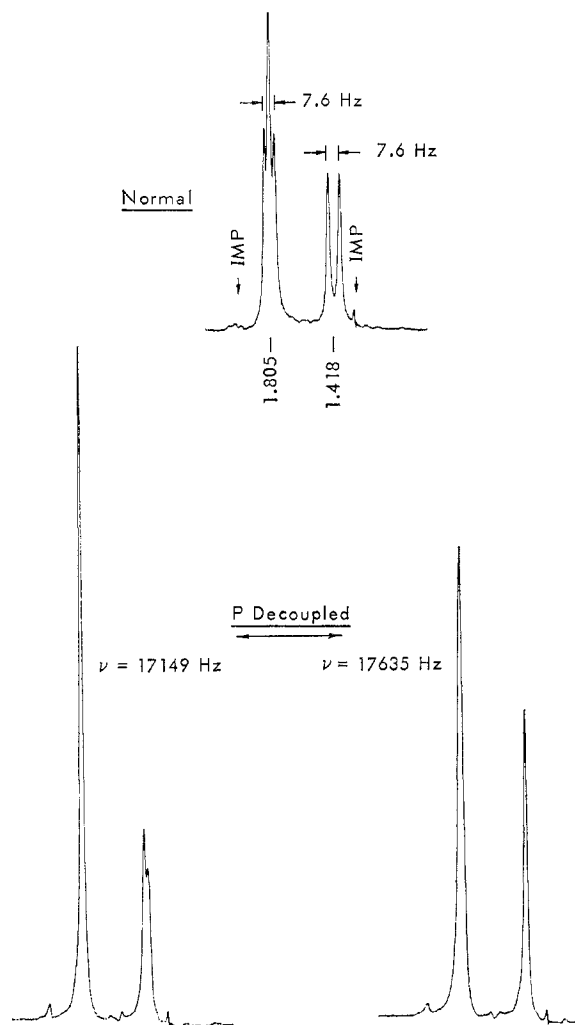
Figure 4.—Nmr spectrum of the methyl region of ((\text{C}_6\text{H}_5)_2\text{PCH}_3)_3(\text{CO})\text{RuH}_2 in \text{C}_6\text{H}_6 at 30^\circ .
