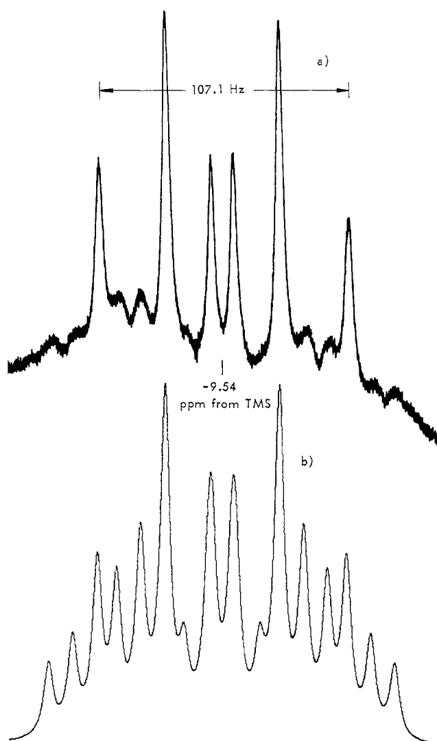
Figure 2.—Nmr spectrum of the hydride region of ((\text{C}_6\text{H}_5)_2\text{PCH}_3)_4\text{RuH}_2 : (a) observed in \text{C}_6\text{H}_5\text{Cl} at 50^\circ ; (b) calculated as a Gaussian distribution (width = 0.5 Hz) of Lorentzian lines (width = 5.0 Hz).
