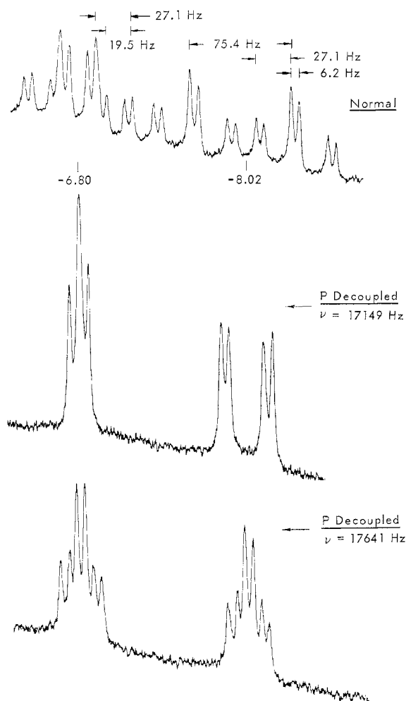
Figure 5.—Nmr spectrum of the hydride region of ((\text{C}_6\text{H}_5)_2\text{PCH}_3)_3(\text{CO})\text{RuH}_2 in \text{C}_6\text{H}_6 at 30^\circ .
