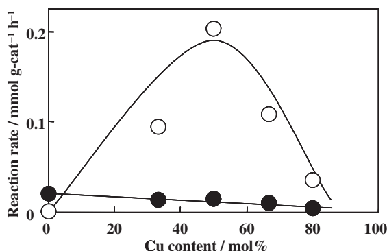
Figure 2. Changes in the reaction rate for the hydrogenation of NO 3 - (○) and NO 2 - (●) in the presence of [Cu m –Pd n ] PVP /AC as function of Cu content. Catalyst: 0.5–1 g, reaction temperature: 333 K, solution of nitrate (200 ppm from NaNO 3 ) or nitrite (148 ppm NaNO 2 ): 0.01–0.06 dm 3 h -1 , H 2 (1 atm): 0.0978 dm 3 h -1 .
