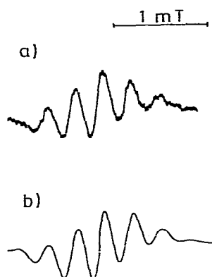
Fig. 5. ESR spectra of \text{PhMe}_2\text{Sn}\cdot : a) observed at -80^\circ\text{C} ; b) calculated with a_{\text{H}}^{\text{CH}_3} = 0.30 mT, a_{\text{O},\text{P}} = 0.05 mT, a_{\text{m}} = 0.03 mT ( \Delta H = 0.125 mT).
