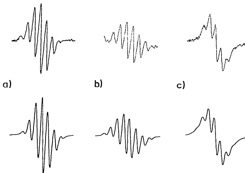
Fig. 6. ESR spectra of tin-centered radicals R_3Sn^\cdot observed (upper portion) and calculated (lower portion). [R_3SnH] = 0.4 M. a) R = \text{neophyl} ( T = 40^\circ\text{C} , \Delta H = 0.125 mT). b) R = \text{methyl} ( T = -80^\circ\text{C} , \Delta H = 0.15 mT). c) R = \text{n-butyl} ( T = -80^\circ\text{C} , \Delta H = 0.25 mT). For splitting parameters see Table 1.
