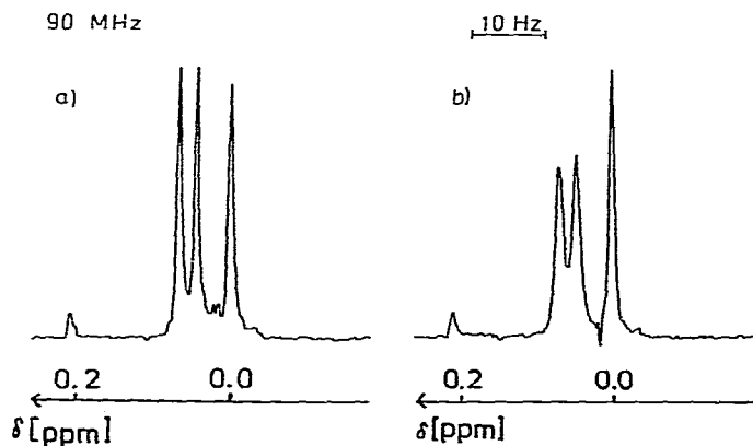
Fig. 2. ^1\text{H} NMR spectra a) without and b) with irradiation of di- t -butyl peroxide with trimethyltin hydride in cyclohexane- d_{12} at 25^\circ\text{C} .
