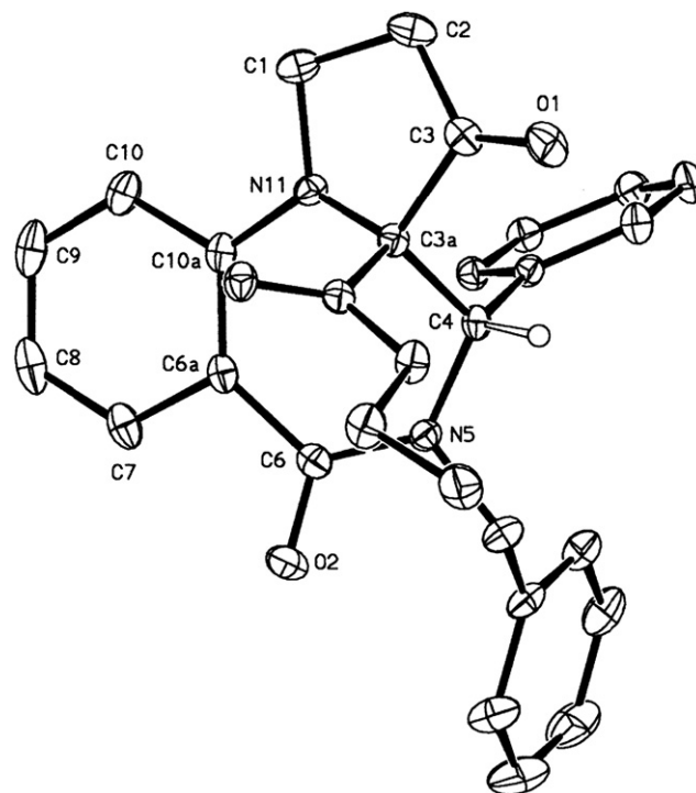
Figure 2. ORTEP view of compound 2e . Hydrogen atoms omitted for clarity: only the hydrogen atom at C-4 is shown.
