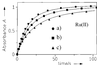
Figure 3. Reduction of [\text{Ru}(\text{phen})_3]^{3+} by bromomalonic acid (concentration of [\text{Ru}(\text{phen})_3]^{3+} versus time curves). Solid lines: experiments with (a) [\text{BrMA}]_0 = 8.0 \times 10^{-4} \text{ M} , [\text{Ru}(\text{III})]_0 = 3.2 \times 10^{-5} \text{ M} , (b) [\text{BrMA}]_0 = 6.0 \times 10^{-4} \text{ M} , [\text{Ru}(\text{III})]_0 = 3.1 \times 10^{-5} \text{ M} , (c) [\text{BrMA}]_0 = 4.0 \times 10^{-4} \text{ M} , [\text{Ru}(\text{III})]_0 = 3.1 \times 10^{-5} \text{ M} . Dots, squares, and triangles: simulated with k_8 = 94.2 \text{ M}^{-1} \text{ s}^{-1} , k_{-8} = 1.1 \times 10^6 \text{ M}^{-2} \text{ s}^{-1} , and k_9 = 1 \times 10^8 \text{ M}^{-1} \text{ s}^{-1} .
