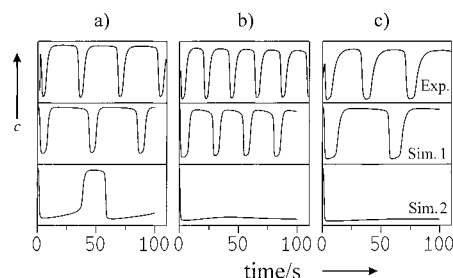
Figure 5. Oscillating system. Concentration c of [\text{Ru(phen)}_3]^{2+} versus time curves (scaling of the ordinate as in Figure 4). Top: experiment. Center: complete model (simulation 1, reactions R1–R16). Bottom: exclusive bromide control model (simulation 2, reactions R1–R12); only one oscillation cycle occurs in case (a), no oscillations occur in cases (b) and (c).
