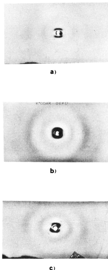
Figure 4. X-ray diffraction patterns of samples aligned by a magnetic field of 1.7 T (X-ray wavelength \lambda (Cu K \alpha ), cylindrical film, Sample-film distance 60 mm): (a) n = 3 , T = 126^\circ\text{C} , nematic phase, exposure time 30 min; (b) n = 15 , T = 100^\circ\text{C} , nematic phase, exposure time 2 h; (c) n = 2 , T = 130^\circ\text{C} , smectic C phase, exposure time 30 min.
