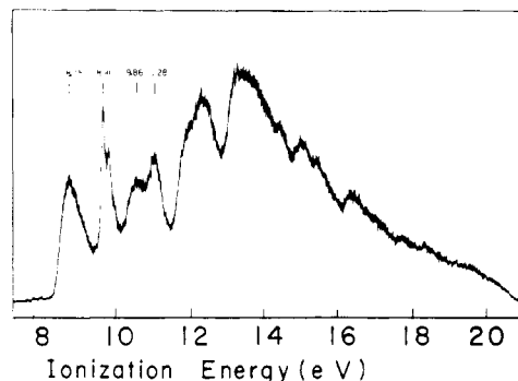
Figure 1. Photoelectron spectrum of 1. 11
