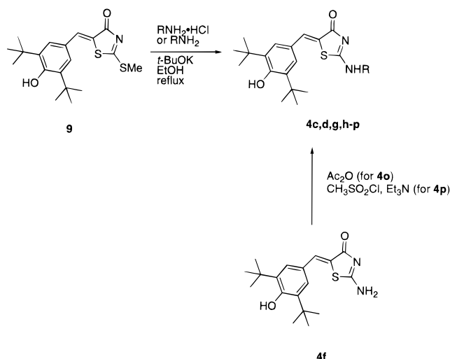
Scheme 3. Preparation of Oxazolone Derivatives
