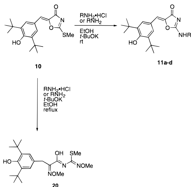
Scheme 3. Preparation of Oxazolone Derivatives
