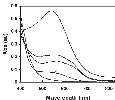
Figure 5. Room temperature UV-vis spectra of 9 in (i) toluene, (ii) \text{CH}_2\text{Cl}_2 , (iii) \text{CHCl}_3 , (iv) \text{CH}_3\text{CN} , and (v) MeOH.
