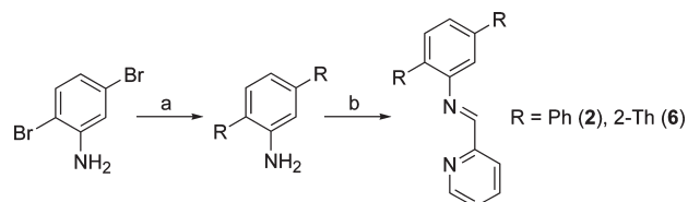
Scheme 2. Preparation of Ligands 2 and 6 a
