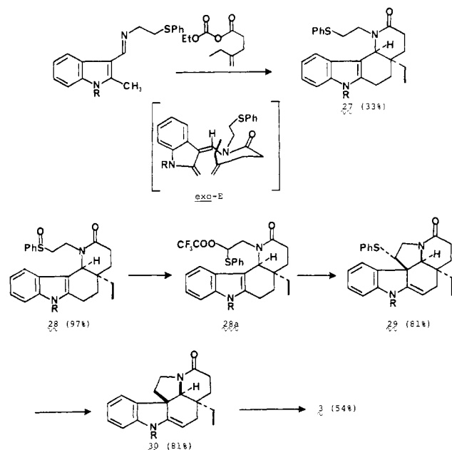
Scheme VI. Endocyclic Amide Route to ( \pm )-Aspidospermidine a
