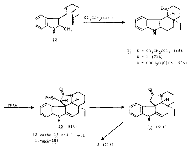
Scheme III. Exocyclic Carbamate Route to (±)-Aspidospermidine a
