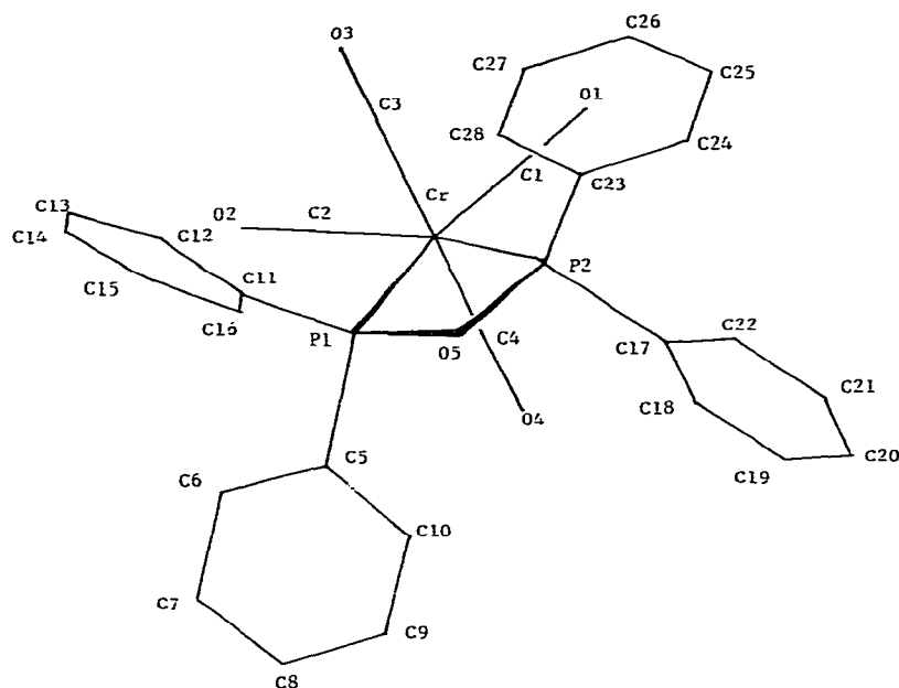
Fig. 1(b). Molecular structure of cis -(CO) 4 Cr(PPh 2 OPPh 2 ).
