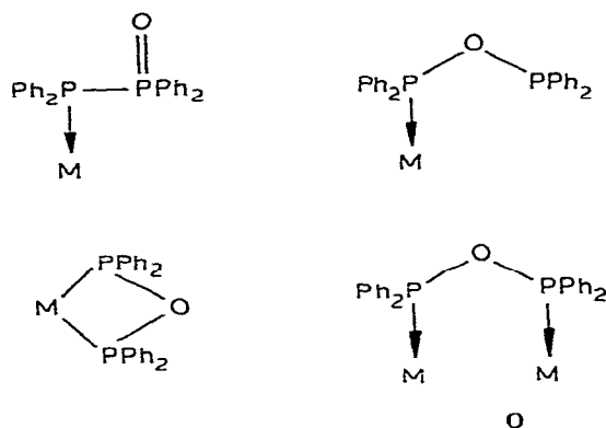
Fig. 4. Known coordination modes of \text{Ph}_2\text{P(=O)Ph}_2 and its tautomer \text{Ph}_2\text{P(OPh}_2\text{)} .
