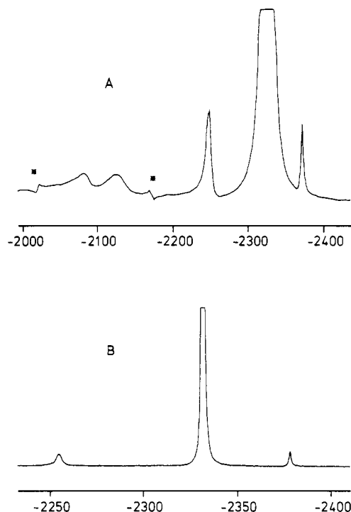
Figure 1. 89.28-MHz ^{55}\text{Mn} NMR spectrum of a mixture of \text{Mn}_2(\text{CO})_{10} (main signal) and \text{Mn}_2(\text{CO})_9\text{CS} , isomers I and II (0.11 M in THF/ \text{THF-}d_8 ): (A) sweep width 125 kHz, time domain 1024K, pulse width 10 \mu\text{s} , relaxation delay 0.5 s (the two peaks indicated with asterisks are due to the scanning technique); (B) section close to the main signal, resolution enhanced, sweep width 45.5 kHz, time domain 8200K.
