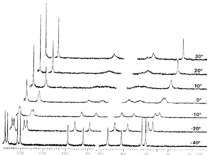
Fig. 3. Variable temperature ^{13}\text{C} NMR spectra of \text{Rh}(\text{COD})(2)_2^+ in \text{CDCl}_3 at 75.43 MHz.
