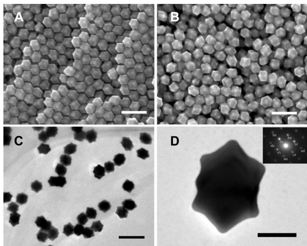
Figure 4. SEM images of (A) orderly assembled and (B) randomly distributed RD gold nanocrystals (scale bars: 200 nm). (C) TEM image of the RD gold nanocrystals (scale bar: 200 nm). (D) TEM image and corresponding SAED pattern of a single flat-lying RD gold nanocrystal recorded along the [011] zone axis (scale bar: 50 nm).
