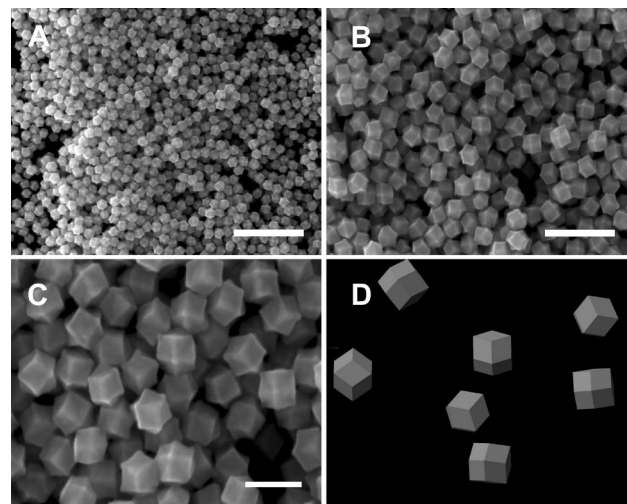
Figure 5. SEM images of larger RD gold nanocrystals at different magnifications [scale bars: (A) 1 \mu m, (B) 500 nm, (C) 200 nm]. (D) RD geometrical models with typical orientations corresponding to RD gold nanocrystals at the same positions in (C).
