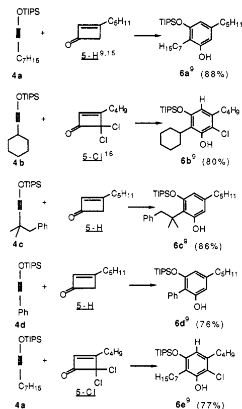
Chart II. Resorcinol Synthesis 13
