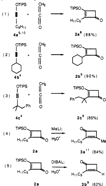
Chart I. Cyclobutenone Synthesis 7
