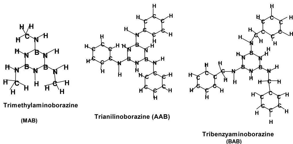
Fig. 1. Aminoborazines used.
