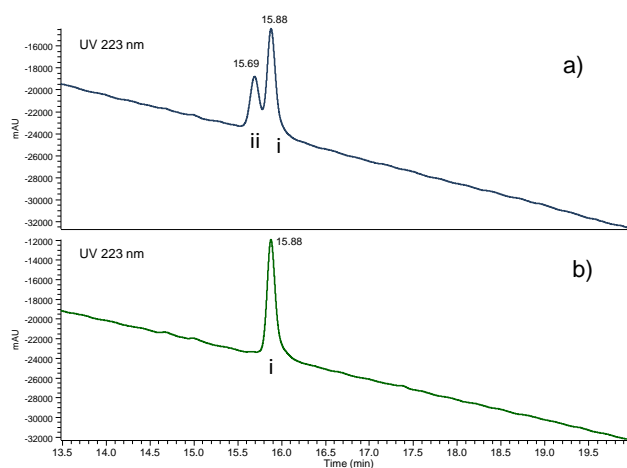
Figure 2. UPLC of SG3249: a) unbuffered TBAF used in Scheme 3, step c; b) buffered TBAF. Ace Excel 2 C18-AR (2 \mu m, 3.0 mm x 100 mm), 40 °C, 20 mM ammonium formate (pH = 4) /acetonitrile, 25/75 to 55/45 over 30 min, 0.6 mL/min. Peaks i and ii in a) Diastereoisomers of SG3249. Peak i in b): pure SG3249.
