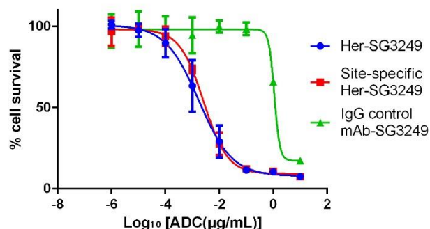
Figure 3. Growth inhibition curves in human SKBR3 cells for SG3249 ADCs.
