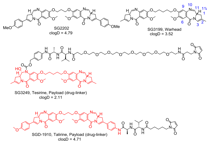
Figure 1. Structures of SG2202 and ADC warhead SG3199. LogD values calculated at pH 7.4. Structures of payloads (drug-linker) SG3249 (tesirine), and SGD-1910 (talirine). Red coding denotes released warhead. Conventional ring numbering shown on SG3199.
