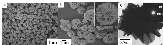
Figure 2. FE-SEM images of the \beta -Ni(OH) 2 flowers (a), inset in Figure 2b was a typical flower; TEM image of a typical flower, inset in Figure 2c was the SAED pattern of a petal.
