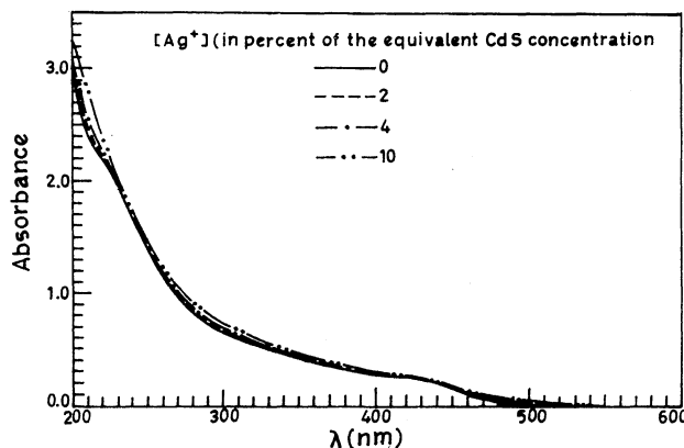
Figure 1(b). Absorption spectra of 0.25 mM CdS containing various concentrations of \text{Ag}^+ (in percent of the equivalent CdS concentration) at pH 10.5: — 0; --- 2; - · - 4; · · · 10.
