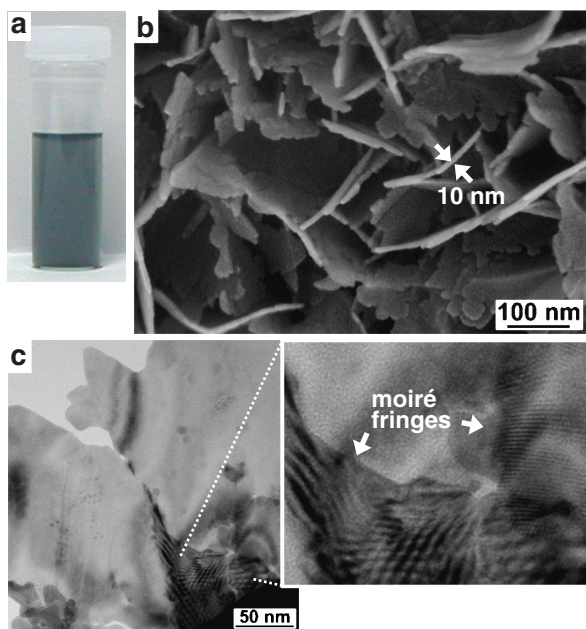
Figure 2. (a) A picture of aqueous dispersion, (b) SEM, and (c) TEM images of ultrathin gold nanosheets. Samples were obtained by photoilluminating mixture of [C_4mim]PF_6 and aqueous Au(OH)_4^- under vigorous stirring.
