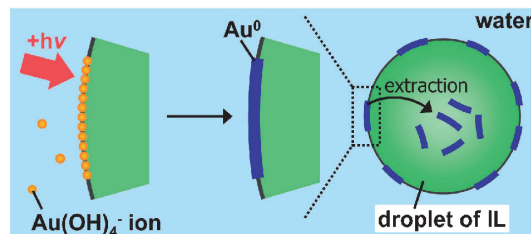
Figure 3. Schematic illustration of the formation of ultrathin gold nanosheets. Photoreduction of Au(III) ions occur at the [C_4mim]PF_6 /water interface and the formed nanosheets are extracted inside the ILs microdroplet. This extraction process prevents the growth in thickness.
