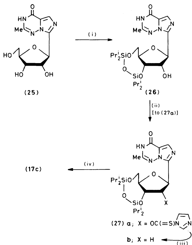
Scheme 2. Reagents: (i) (\text{Pr}_2\text{SiCl})_2\text{O} -pyridine; (ii) (\text{imidazol-1-yl})_2\text{C=S} -DMF; (iii) \text{Bu}_3\text{SnH} -AIBN-toluene; (iv) \text{Bu}_4\text{N}^+\text{F}^- -THF
