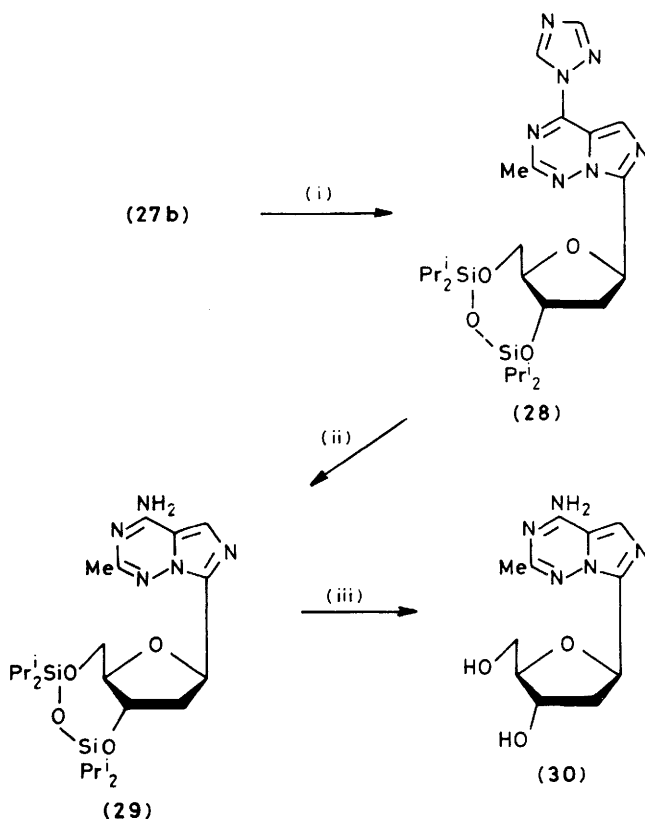
Scheme 3. Reagents: (i) \text{POCl}_3 - \text{Et}_3\text{N} -1,2,4-triazole; (ii) \text{NH}_3 -THF; (iii) \text{Bu}_4\text{N}^+\text{F}^- -THF
