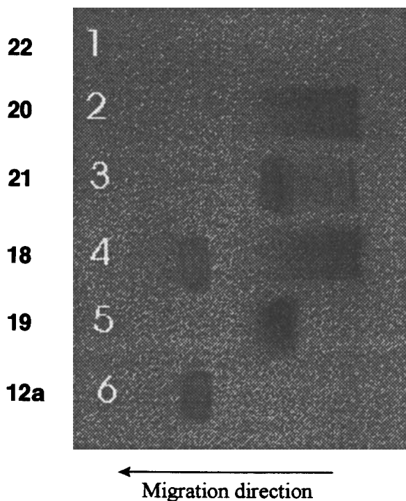
Fig. 2. Non-denaturing 21% polyacrylamide gel electrophoresis of the oligomers 12a and 18–22 after incubation of 0.6 A_{260} units with 0.1\text{ M NaCl} . For conditions, see Exper. Part .
