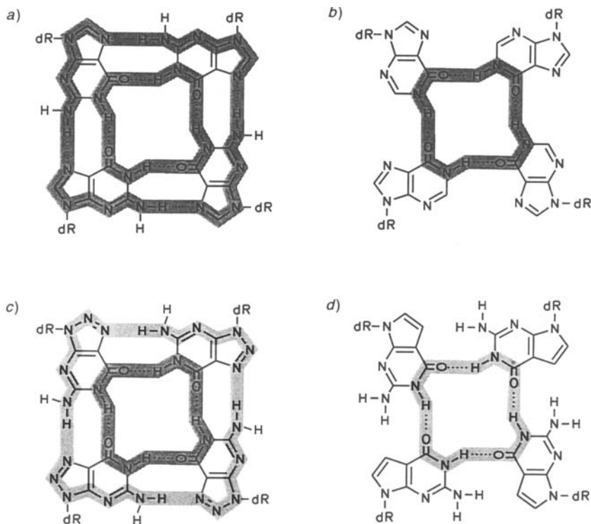
Fig. 4. Tetrameric structures a) proposed for d(T-G-G-G-T) ( 18 ), b) of oligo( I_d ) [32], and c) d) proposed for d(T-z^8G-z^8G-z^8G-T) ( 19 ) and d(T-c^7G-c^7G-c^7G-T) , respectively. dR = 2'-Deoxyribsyl.
