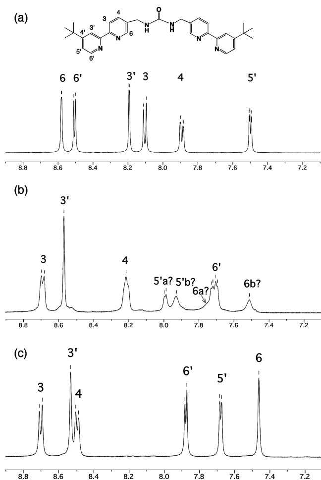
Figure 3. Aromatic regions of the ^1\text{H} NMR spectra of (a) free t BuL1, (b) [\text{Zn}_2(\text{tBuL1})_3](\text{NO}_3)_{4n} , and (c) [\text{Zn}_4(\text{tBuL1})_6](\text{SO}_4)(\text{NO}_3)_6 in 2:1 \text{CD}_3\text{OD}-\text{D}_2\text{O} .
