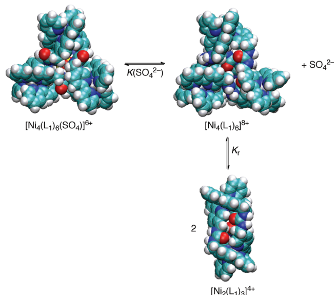
Scheme 2. Putative Reaction Equilibria Involving the [Ni 4 (L1) 6 (SO 4 )] 6 6+ Cage in Aqueous Solutions a
