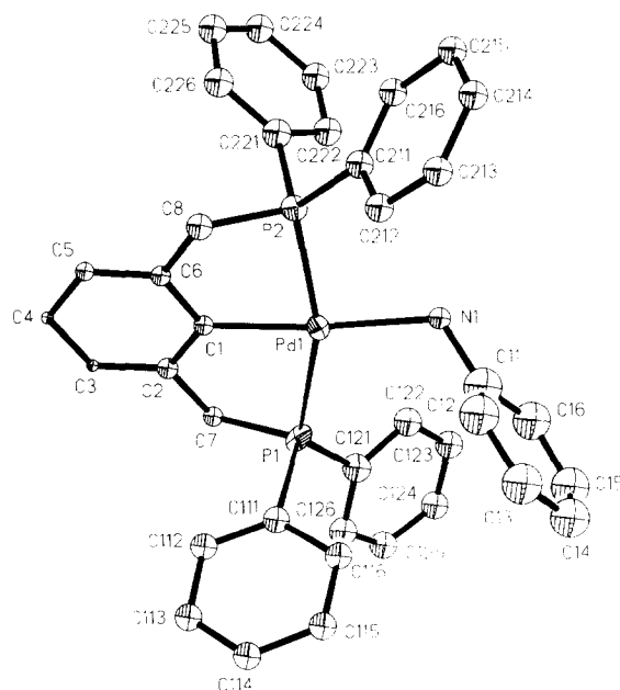
Fig. 2. ORTEP [20] drawing of the cation [(dppx)PdNH 2 Ph] + .
