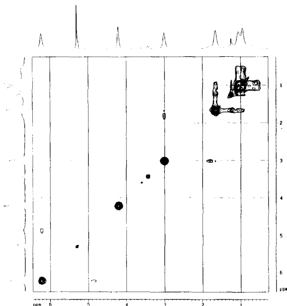
Fig. 1. NOESY spectrum of 7 in \text{CDCl}_3 in the presence of free THF ( 20^\circ\text{C} , \tau_{\text{mix}} = 0.1 s).
