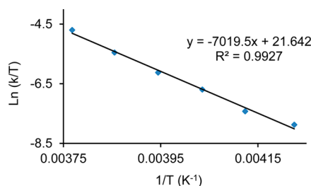
Figure 5. Eyring plots for the dynamic processes observed by ^1\text{H} NMR in \text{tol-}d_8 for complex 7b .
