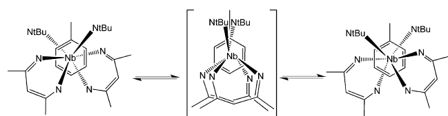
Scheme 6. Proposed Dynamic Processes Observed in Solution for Complex 7b
