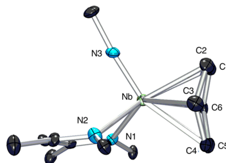
Figure 1. Thermal ellipsoid plot of the complex 2a . Diisopropyl aryl groups of the BDI ligand have been removed, and ^tBu moieties have been truncated for clarity. Full structure and structural parameters are presented in the SI.
