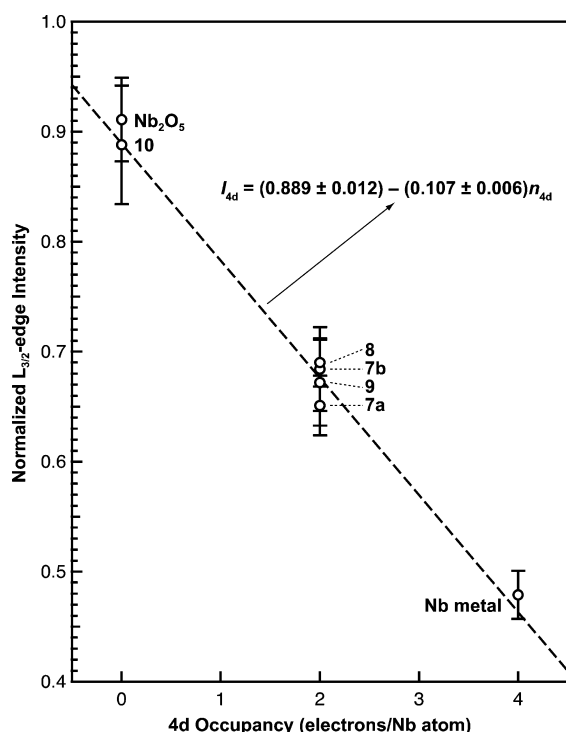
Figure 8. A plot of normalized L_{3,2} -edge intensity vs 4d occupancy of 7a–b , 8 , 9 , 10 , \text{Nb}_2\text{O}_5 , and Nb metal. Error bars are taken from the standard deviation in the intensities determined over repeated measurements. A linear fit to all data (dashed line) gives the equation shown.
