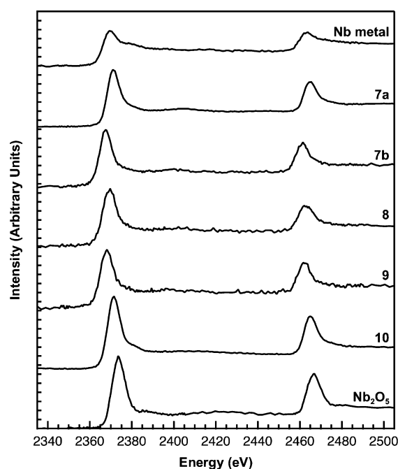
Figure 7. Representative background-subtracted Nb L_{3,2} -edge XANES spectra for compounds 7a–b , 8 , and 9 . Also included are reference materials 10 , Nb metal, and \text{Nb}_2\text{O}_5 . All data was collected using a STXM.
