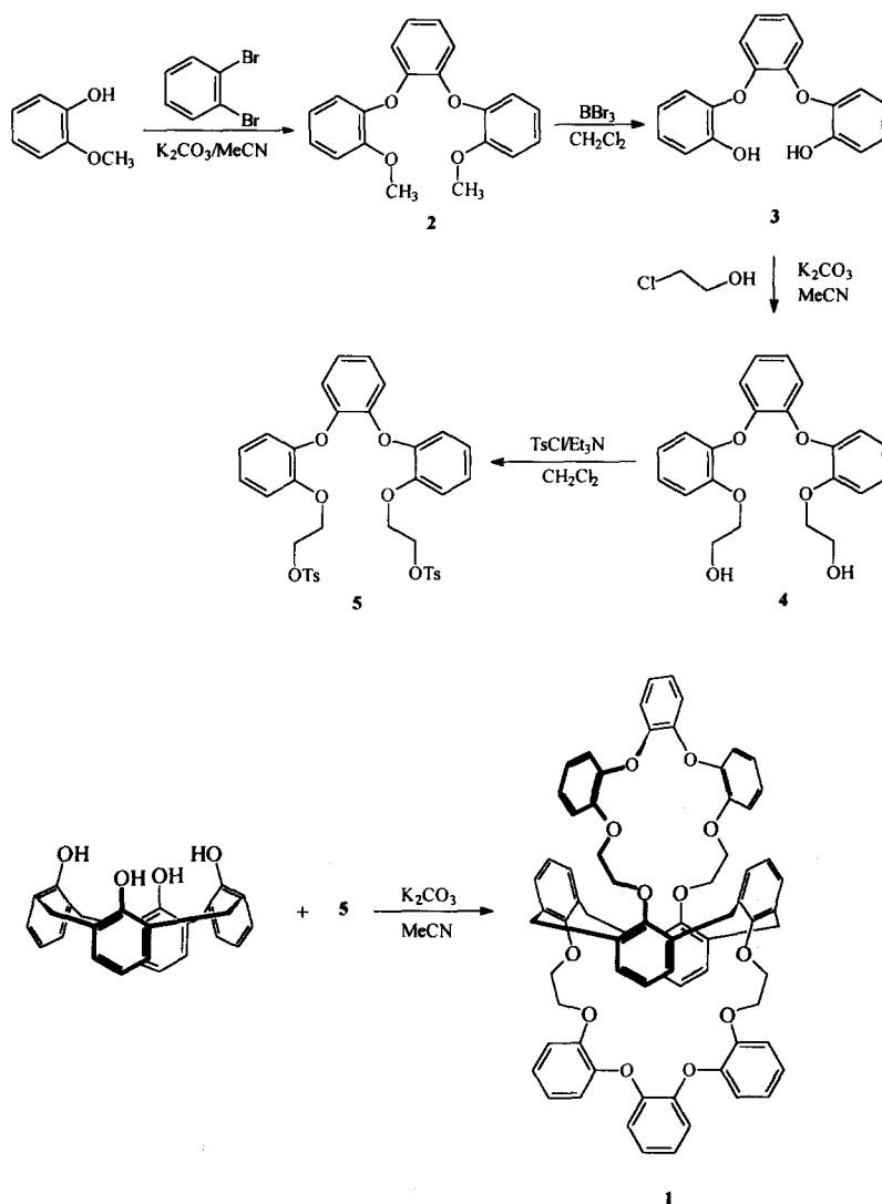
Scheme 1. Synthesis of 1
