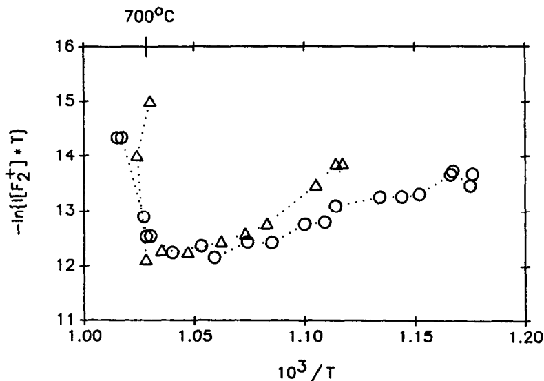
Fig. 3 - Results of mass spec. studies of \text{AmF}_4 : \circ = F_2^+/\text{AmF}_4\text{-I} ; \Delta = F_2^+/\text{AmF}_4\text{-II} .
