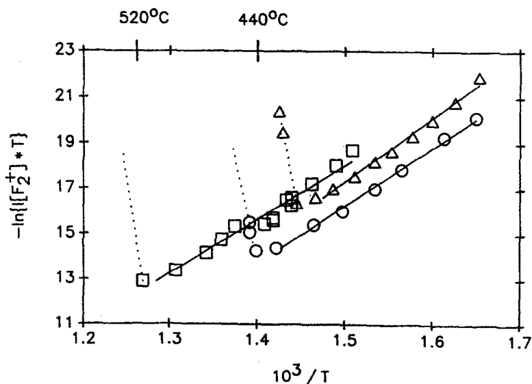
Fig. 2 - Results of mass spec. studies of \text{CmF}_4 and \text{TbF}_4 : ○ = \text{F}_2^+/\text{CmF}_4\text{-I} ; △ = \text{F}_2^+/\text{CmF}_4\text{-II} ; □ = \text{F}_2^+/\text{TbF}_4\text{-I} .
