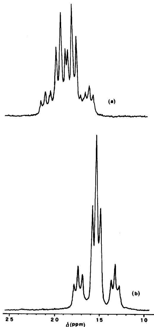
Fig. 2. The \delta(\text{P-Me}) resonance patterns of (a) \text{trans-}[\text{PtBr}(2\text{-pyH})(\text{PMe}_2\text{Ph})_2]\text{ClO}_4 (XIV) and (b) \text{trans-}[\text{PtBr}(2\text{-py})(\text{PMe}_2\text{Ph})_2] in \text{CD}_2\text{Cl}_2 at 30^\circ\text{C} .
